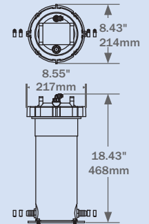
Commercial Pre-Filter / OW Separator
