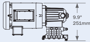
HP Pump (200 & 360)
