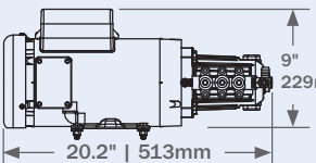
HP Pump (600 & 800)
