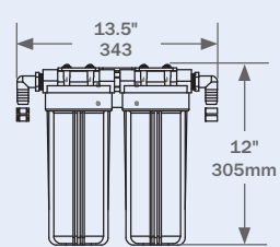
Dual Pre-Filter
