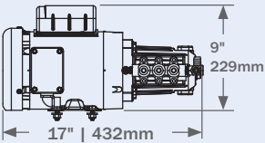
HP Pump (200 & 360)
